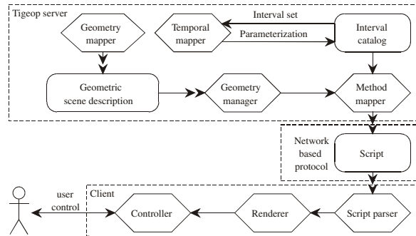
Figure 1. Overview of the TIGEO-based client/server architecture for hybrid presentation systems.
