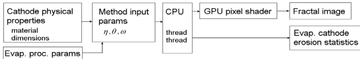
Figure 2. Data flowchart.
