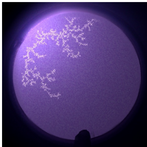
Figure 3a. Cathode spot walk fractal model containing 1200 particles ( \eta = 1 ).
