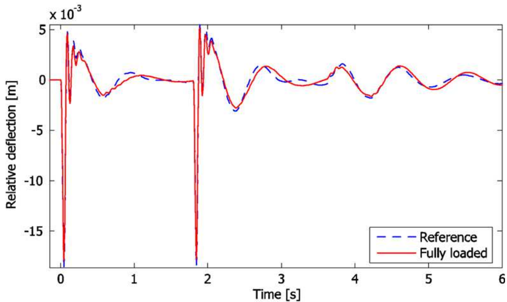
Fig. 9. Time histories of relative deflections of the right front air spring of the fully loaded bus and of the bus of the reference load (comparison of the reference case with the optimally tuned force-velocity characteristics)
