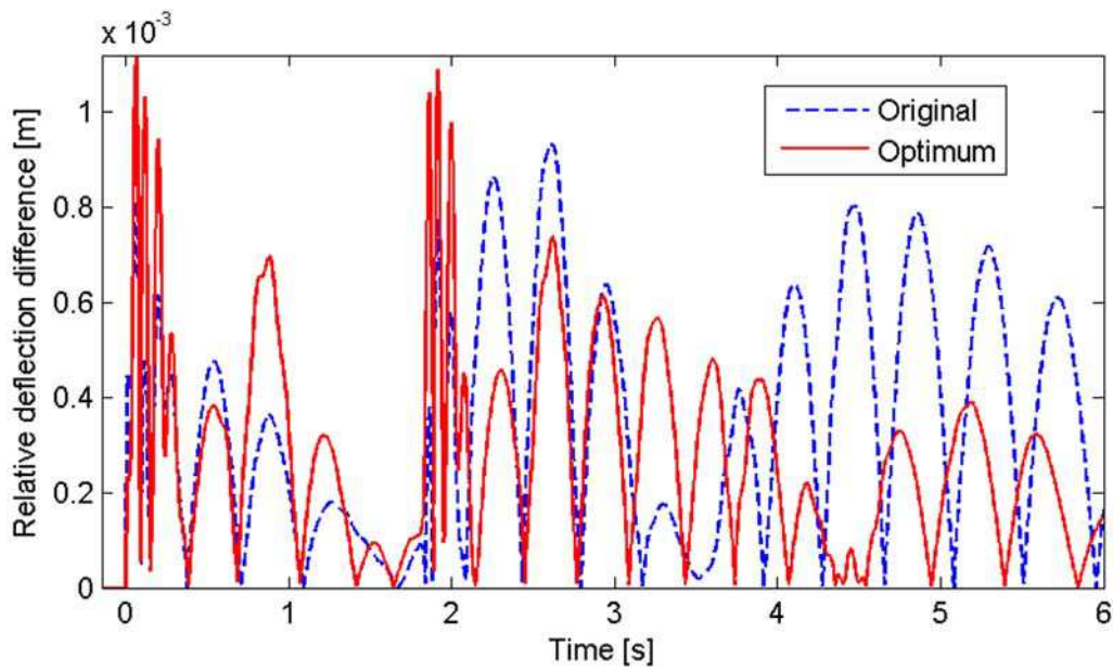
Fig. 10. Differences of time histories of relative deflections of the right front air spring of the fully loaded bus and of the bus of the reference load (comparison of the original and the optimally tuned force-velocity characteristics)
