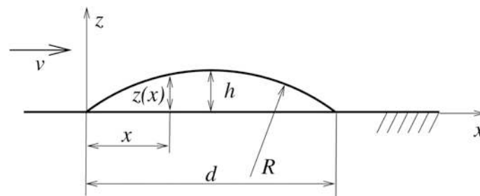
Fig. 5. The standardized artificial obstacle
