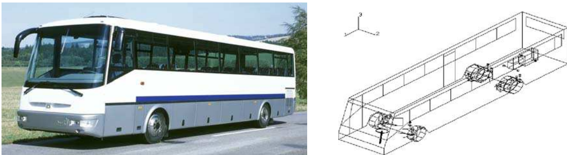
Fig. 2. The SOR C 12 intercity bus — the real vehicle and the multibody model visualization
