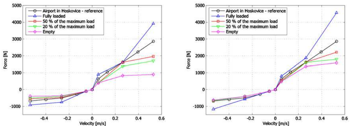
Fig. 12. The originally designed [12, 14] and the verified force-velocity characteristics of the APCSA of the rear axle of the SOR C 12 intercity bus
