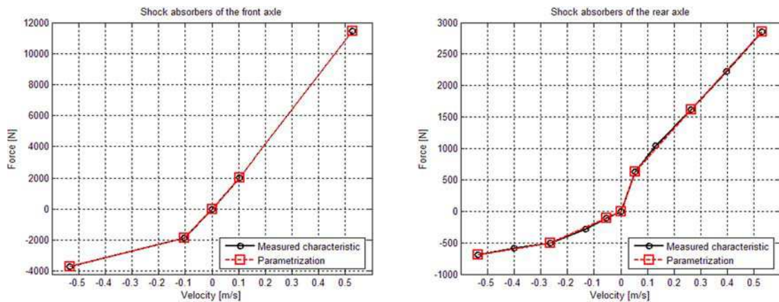
Fig. 3. The force-velocity characteristics of non-controlled shock absorbers of the front and rear axles of the SOR C 12 intercity bus and their parametrization
