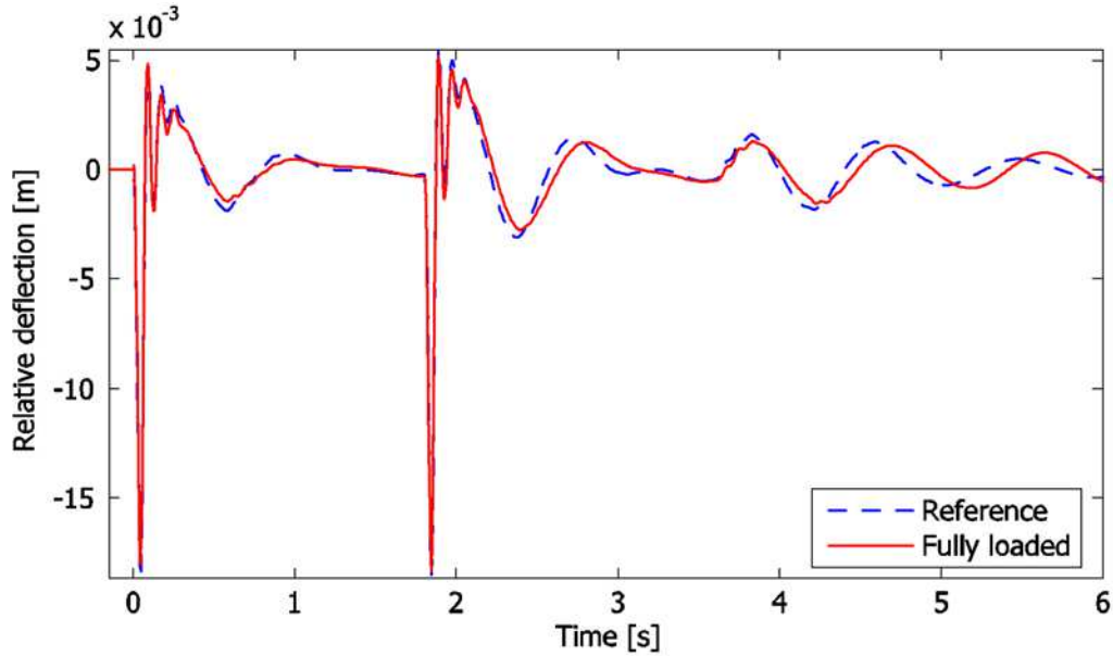
Fig. 8. Time histories of relative deflections of the right front air spring of the fully loaded bus and of the bus of the reference load (comparison of the reference case with the original force-velocity characteristics)
