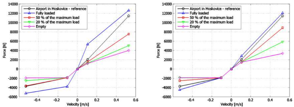
Fig. 11. The originally designed [12, 14] and the verified force-velocity characteristics of the APCSA of the front axle of the SOR C 12 intercity bus
