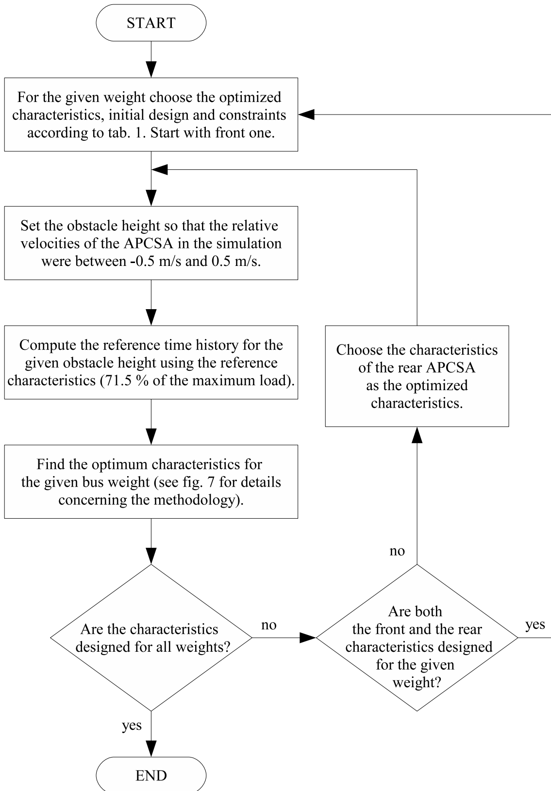
Fig. 6. The methodology of the design of the APCSA optimum characteristics
