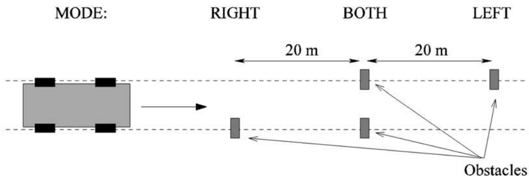
Fig. 4. Scheme of the track according to the ŠKODA VÝZKUM road vehicles testing methodology
