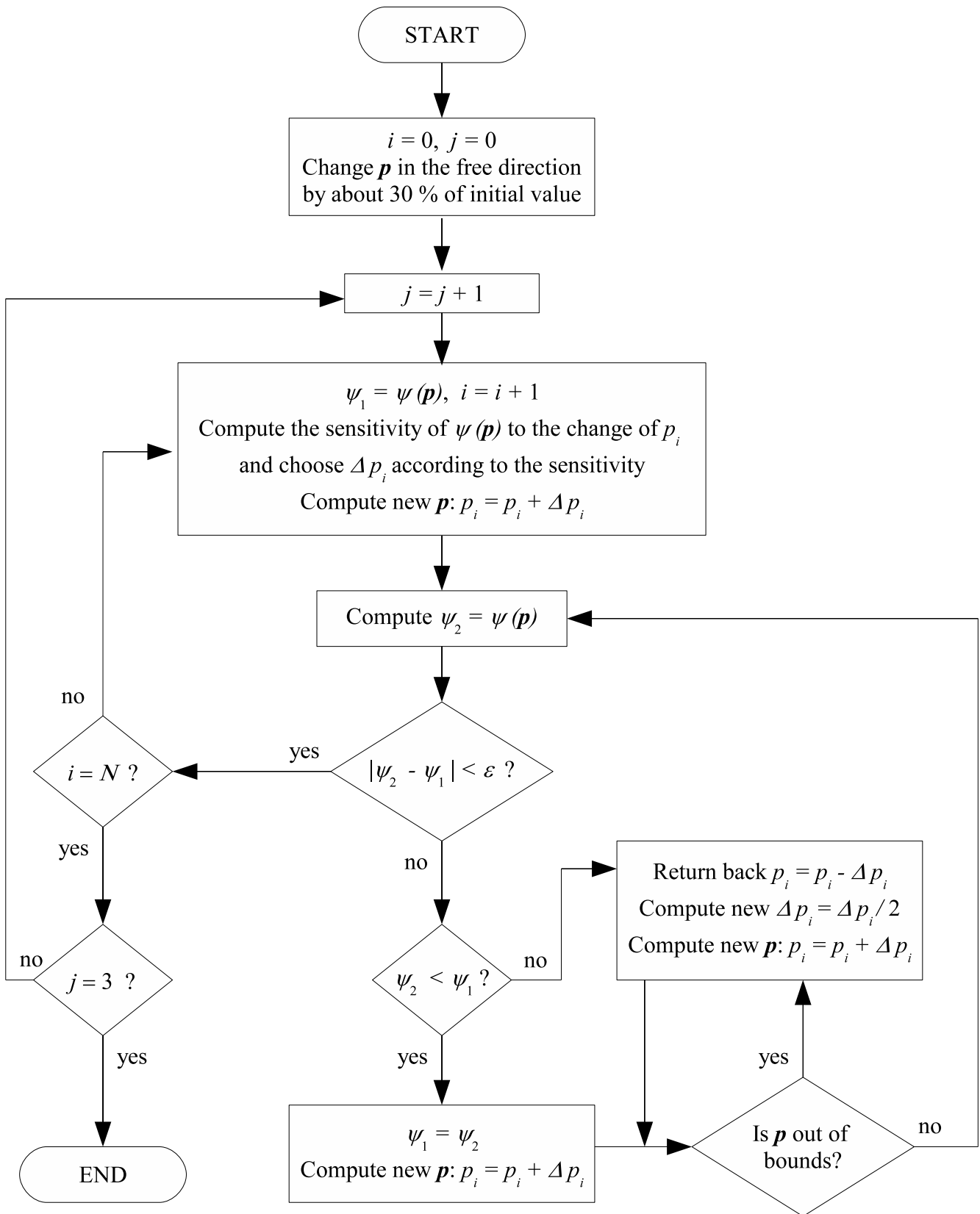
Fig. 7. The optimization methodology for the design of the APCSA characteristics for the given bus weight
