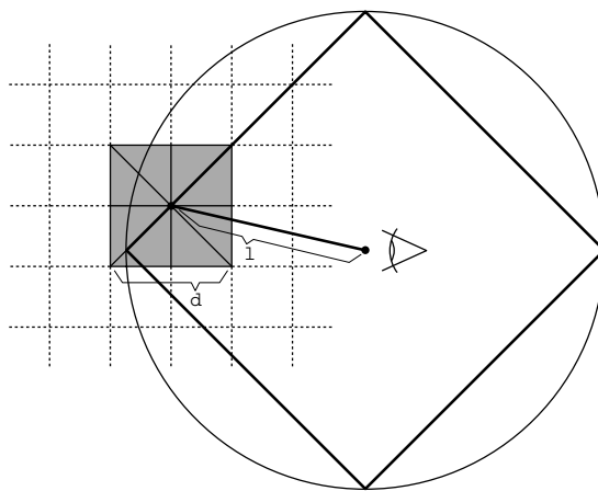
Figure 3: Global resolution criterion: distance versus size of quadtree cells.
