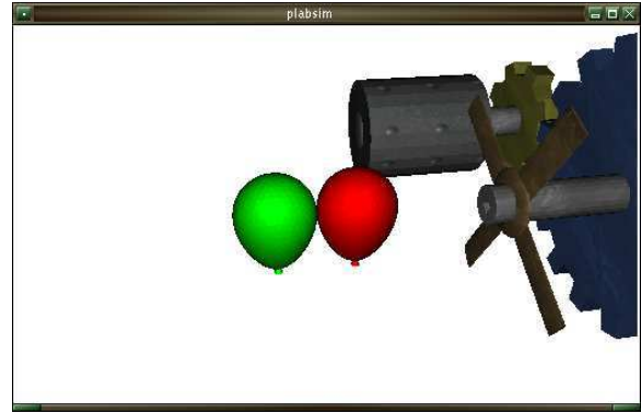
Figure 9. Collision time.
