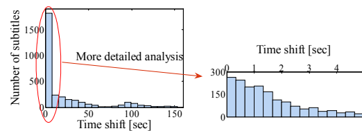
Fig. 5. Histogram: speech utterances desynchronisation for the MM synthesizer.
