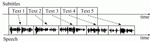
Fig. 3. The origin of the synthesized speech desynchronisation.
