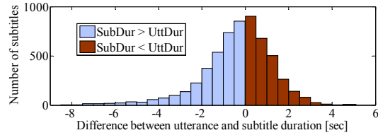
Fig. 4. Histogram: difference between subtitle durations (SubDur) and corresponding synthesised speech utterances (UttDur) for the MM synthesizer.
