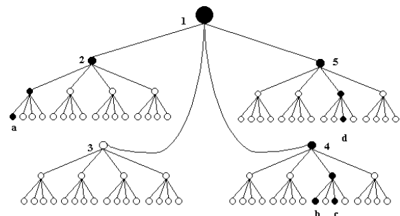
Figure 3 Significance map Or-tree for the sub-band in figure 2; black circle represents a significant node while white circle represents an insignificance node.
