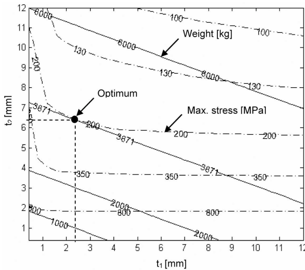
Fig. 4. Graphic presentation of the optimizing problem
