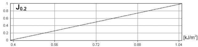
Fig. 9. Distribution function of the J_{0,2} integral
