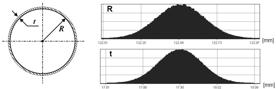
Fig. 6. Histograms of piping geometrical parameters
