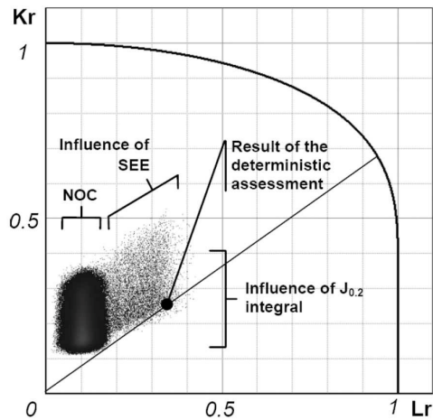
Fig. 15. The “Anthill” diagram
