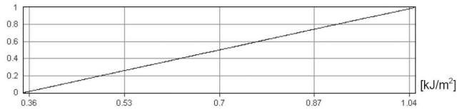
Fig. 3. Distribution function of the J_{0,2}
