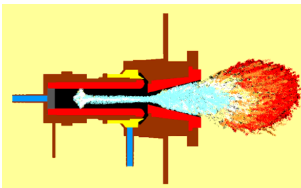
Fig.2: Chart of generator of low-temperature plasma [4]
