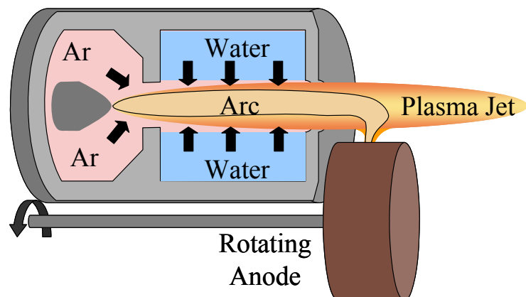
Fig.4: Char of hybrid plasma generator
