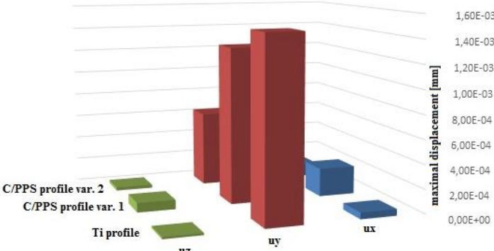
Fig. 3. Comparison of for all cases of clamped T-profiles
