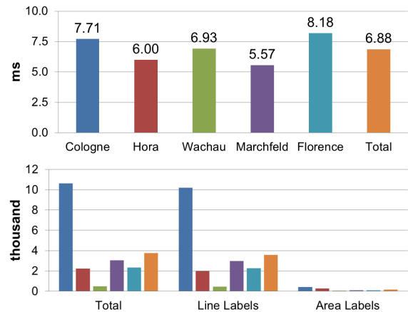
Figure 9: The average time needed for one render pass per case study (top). The number of line and area labels and the total number of labels per case study (bottom).
