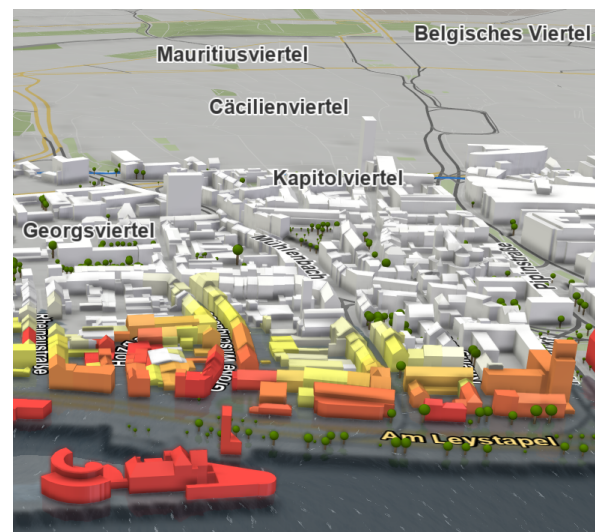
Figure 1: Integration of area and line labels into an interactively explorable and dynamically changing 3D environment with rising water.
