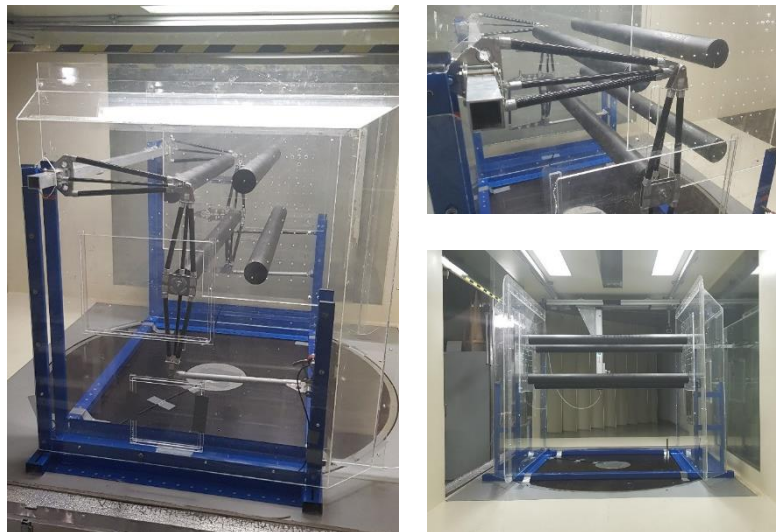
Fig. 2. Experimental set-up with mounted cylinders represented a real configuration of hangers
