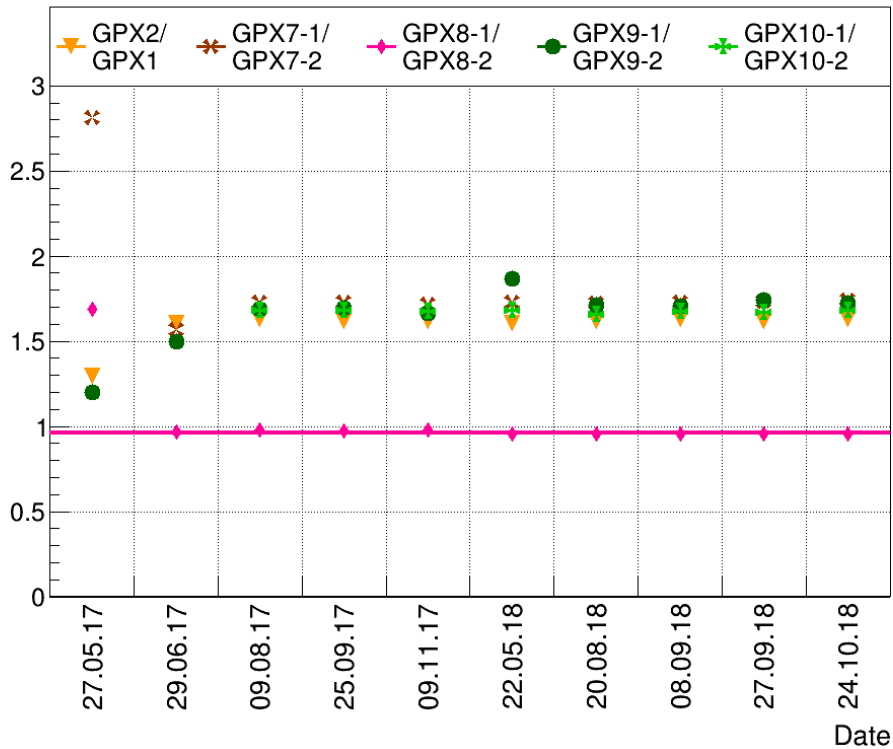
Figure 8. Ratio of cluster (event) counts of thick (1000 \mu\text{m} ) to thin (500 \mu\text{m} ) GaAsPix sensor layers at the same location in the ATLAS cavern.
