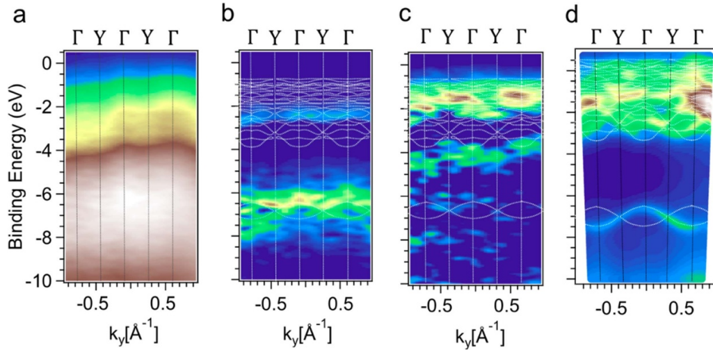
Figure 5. Experimental and theoretical \Gamma Y\Gamma valence band dispersion of PEPI. (a) ARPES raw data (b) after 2D curvature analysis (c) normalized to the density of states and followed by a 2D curvature analysis. (d) Theoretical simulation of the ARPES data, with broadening the band, including SOC and considering only the inorganic part of the crystal. The theoretical band structures are superimposed on the experimental and theoretical spectra of ARPES. The flatter dispersion in the experimental results could be due to the strong electronic localization and quantum confinement in the real system.
