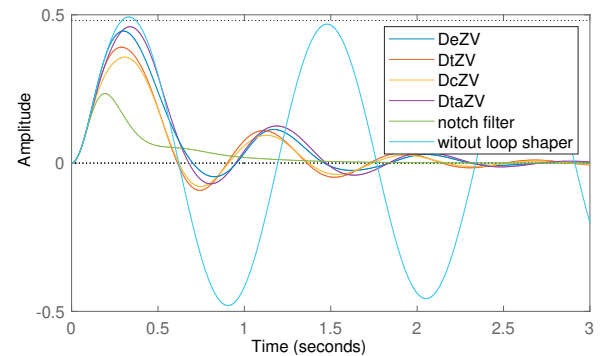
Fig. 10. Closed-loop load-side position response to step output disturbance change, inverse shaper structure
