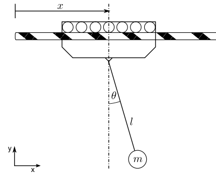
Fig. 4. Gantry crane anti-sway problem
