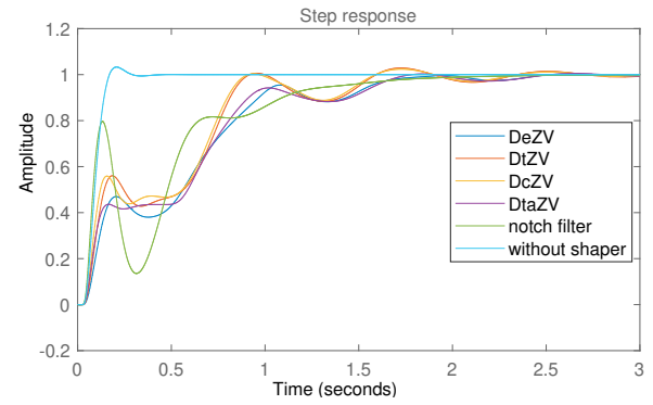
Fig. 8. Closed-loop actuator-side position response to step reference change, inverse shaper structure
