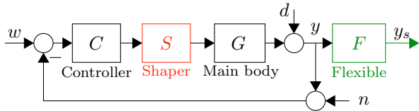
Fig. 2. Feedback loop with control-action shaper
