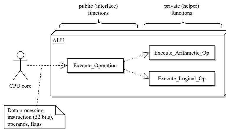
Figure 6.34: Architectural structure of the ALU
