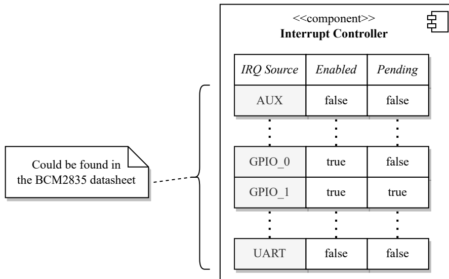
Figure 6.22: Encapsulated information about IRQ sources
