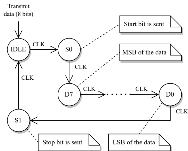
Figure 6.27: Mini_UART state machine (transmitting 8 bits)
