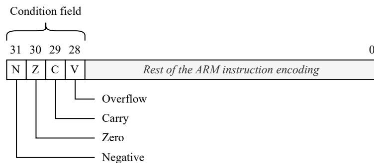
Figure 3.7: Condition field of an ARM instruction
