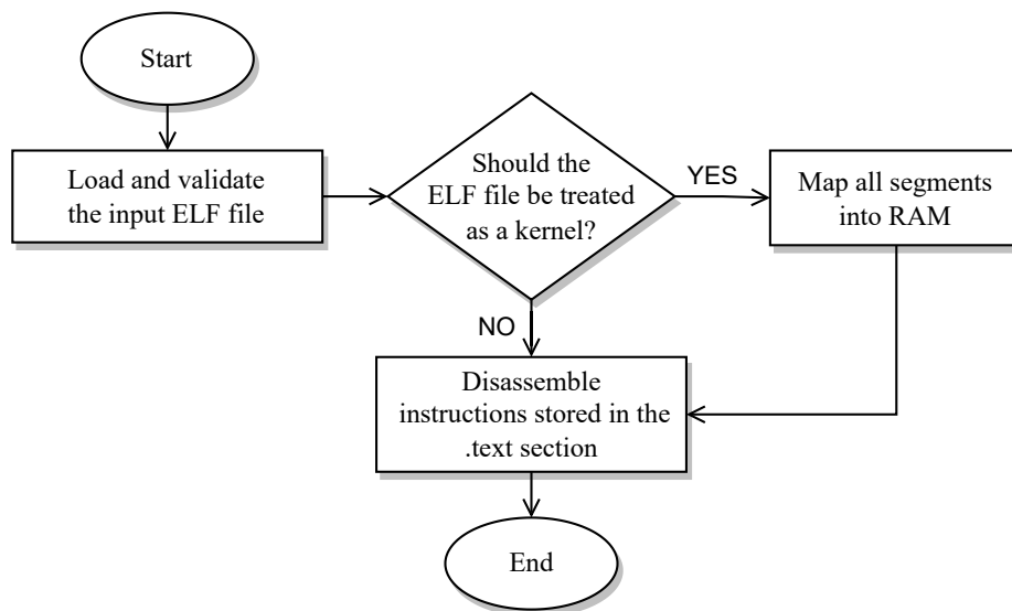
Figure 6.9: Internal logic of the ELF Loader component
