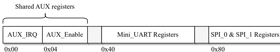
Figure 6.23: Registers of the AUX peripheral
