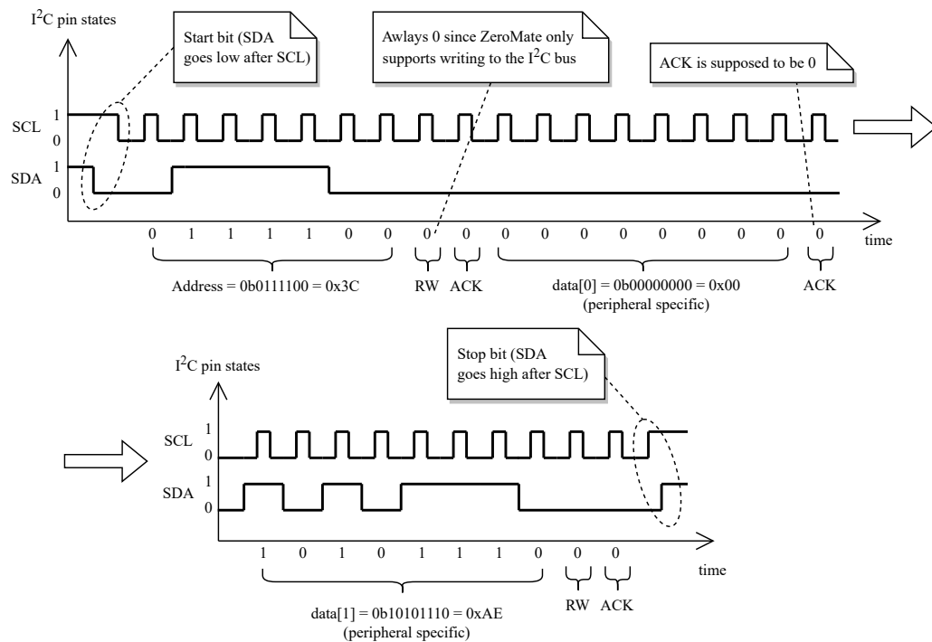
Figure 6.28: Structure of an I 2 C frame
