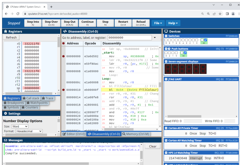
Figure 5.2: CPUlator
