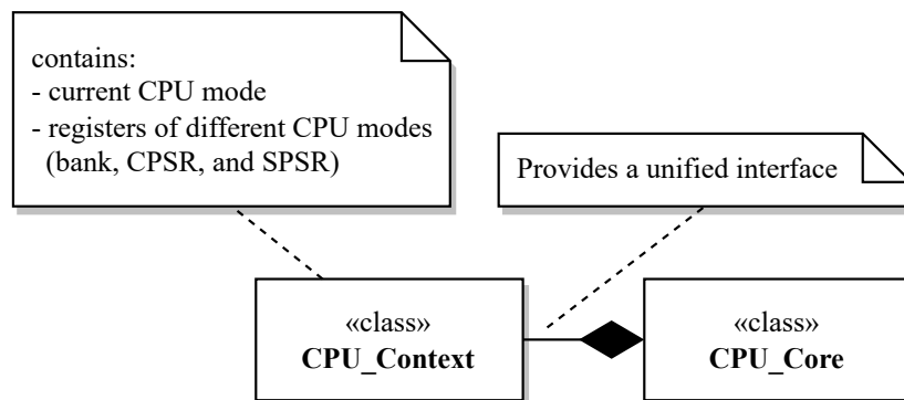
Figure 6.30: Relationship between the CPU context and the CPU core
