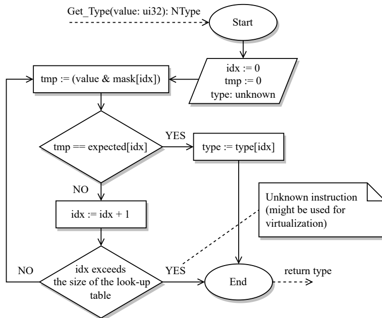
Figure 6.32: Algorithm for decoding ARM instructions
