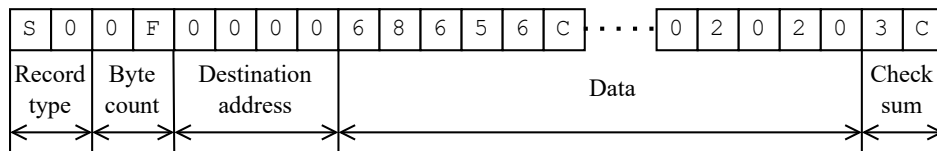
Figure 6.1: Single SREC record (16-bit addressing)
