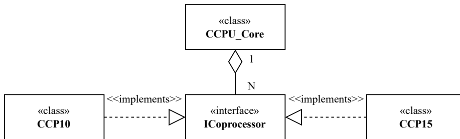
Figure 6.39: Co-processor hierarchy
