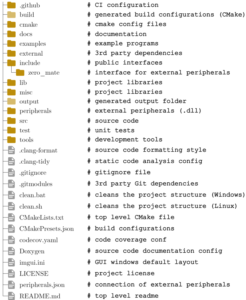
Figure 12.1: ZeroMate project structure
