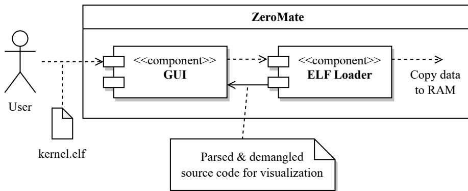
Figure 6.8: Loading an input ELF file (kernel)
