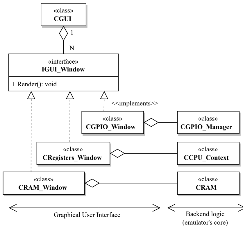
Figure 6.45: Structure of GUI windows
