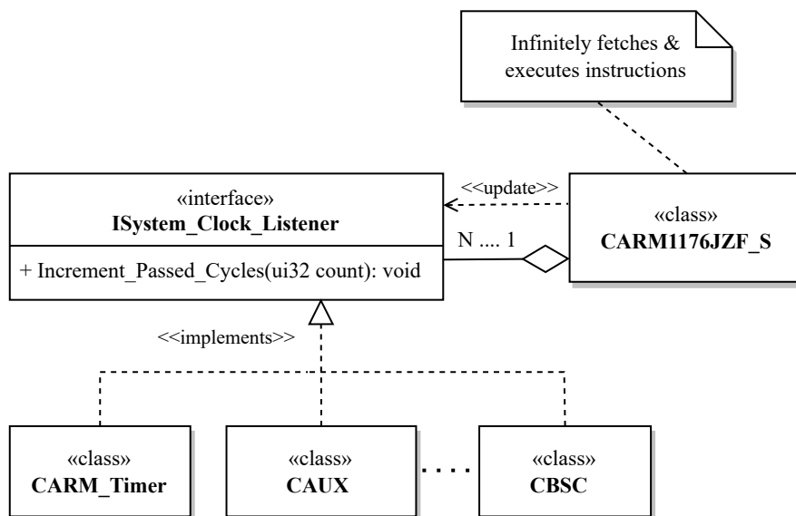
Figure 6.14: ISystem_Clock_Listener interface
