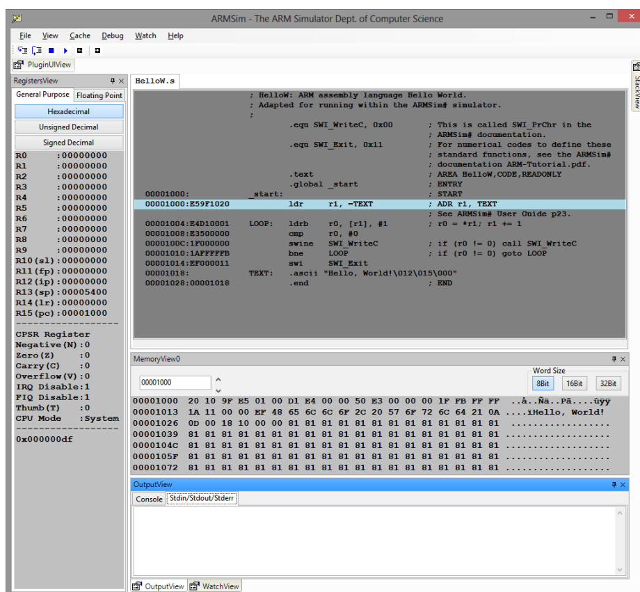
Figure 5.3: ARMSim#
