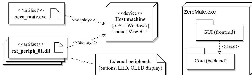
Figure 6.4: Deployment diagram of the ZeroMate emulator
