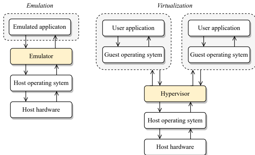
Figure 5.1: Emulation vs. virtualization
