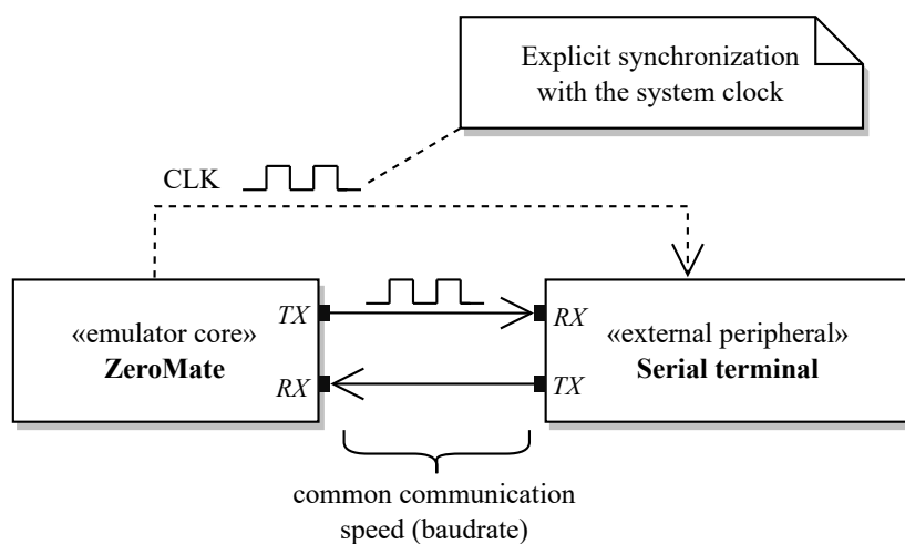
Figure 6.25: UART communication with an external peripheral
