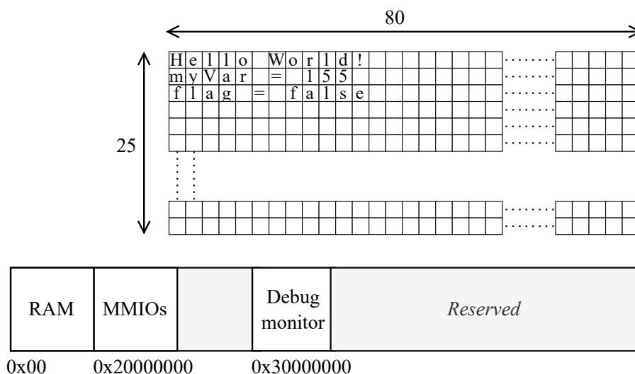
Figure 6.16: Memory-mapped debug monitor
