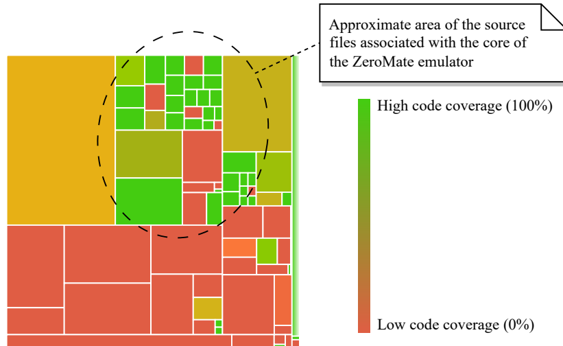
Figure 8.2: Code coverage of individual source files (exported from Codecov [42])
