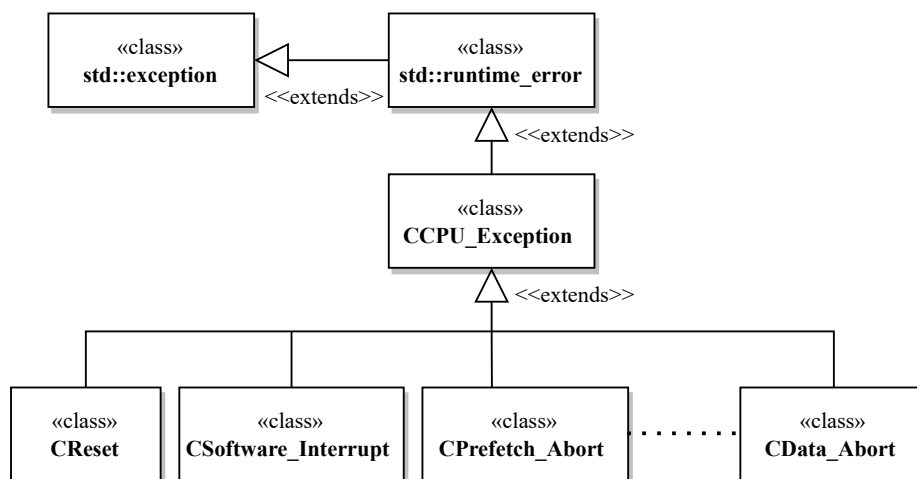
Figure 6.33: Hierarchy of the CPU exceptions
