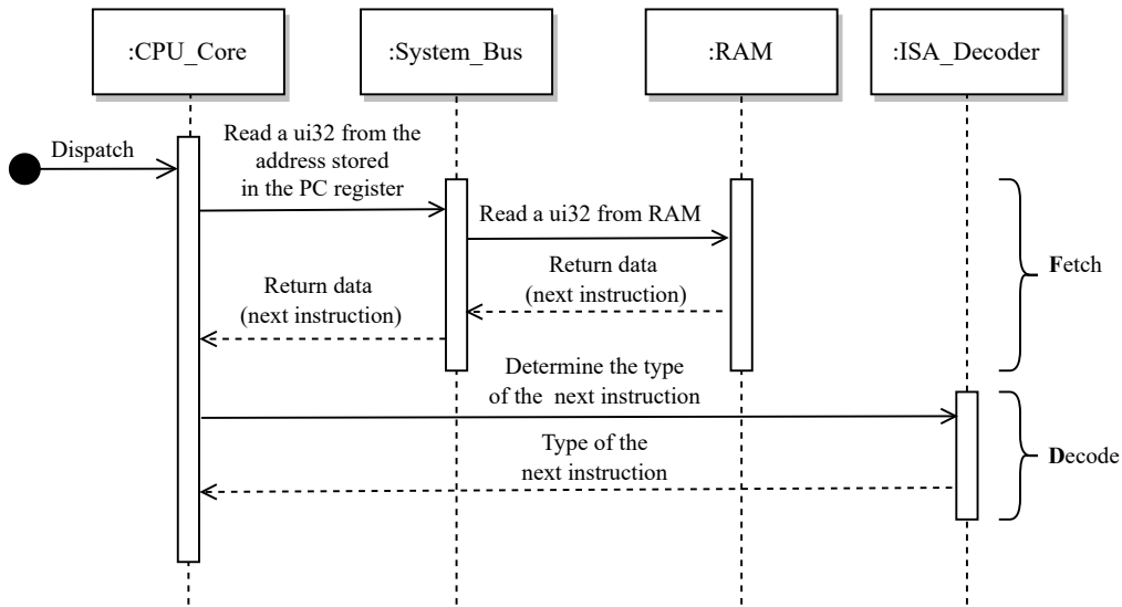
Figure 6.31: Use of the ISA decoder by the CPU
