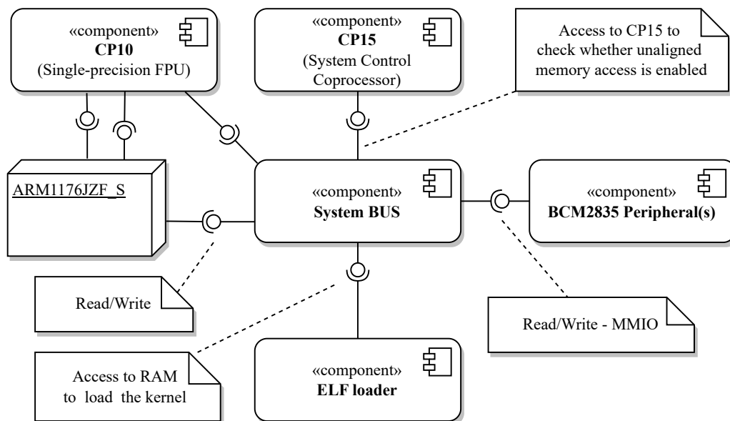
Figure 6.5: Core components of the ZeroMate emulator
