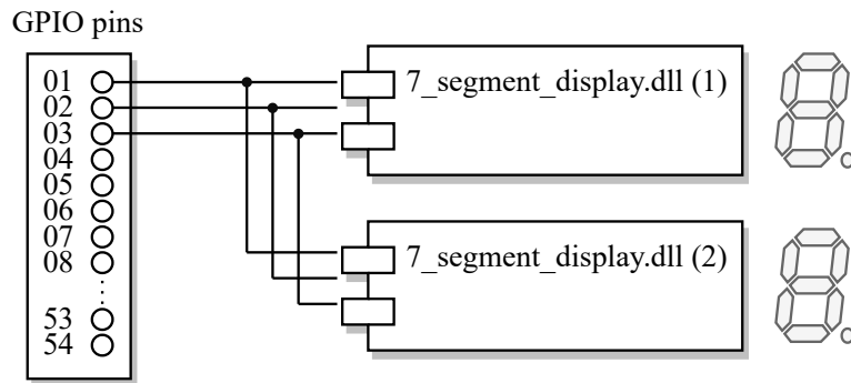
Figure 6.42: Illustration of connection of two parallel 7-segment displays
