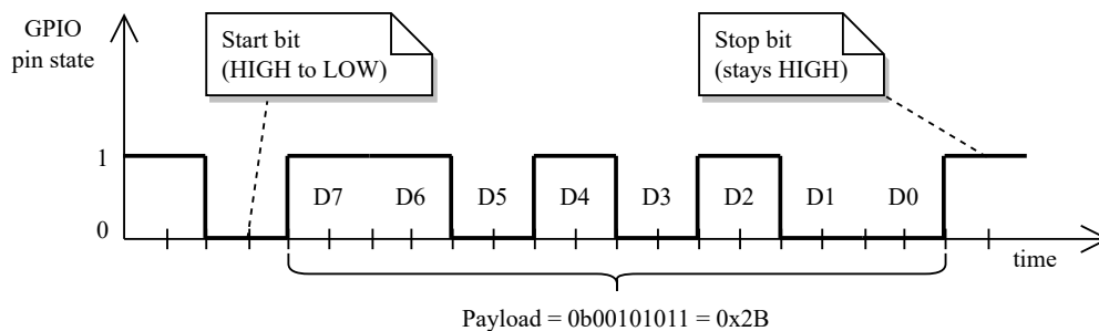
Figure 6.26: Example of a Mini_UART data frame with 8 bits of data
