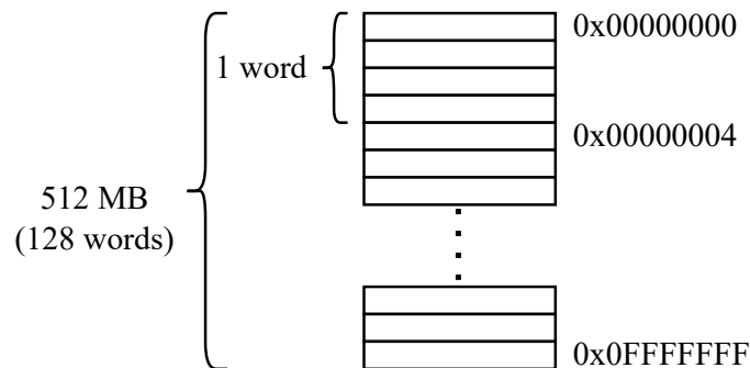
Figure 6.15: RAM implementation as a continuous piece of memory
