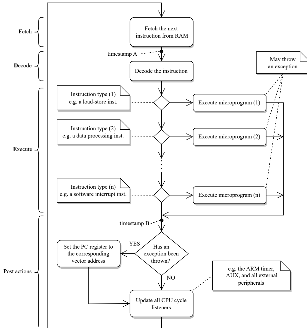
Figure 6.37: Execution loop of the emulated CPU 20
