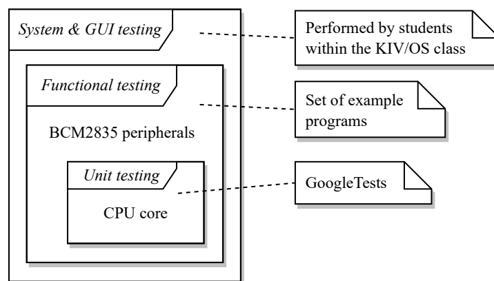
Figure 8.1: Testing strategy leveraged in the ZeroMate project
