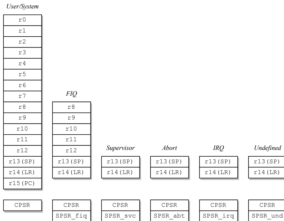
Figure 3.5: Bank registers of different CPU modes
