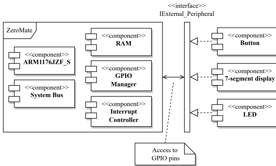
Figure 6.10: Internal vs External peripherals
