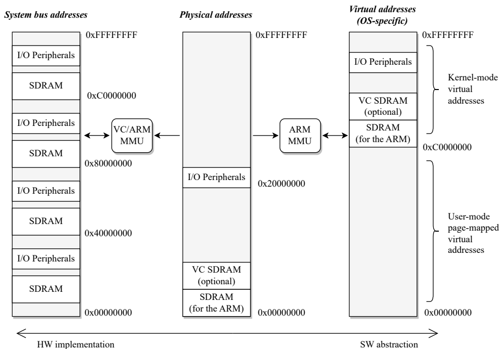
Figure 4.2: BCM2835 address translation processes 3
