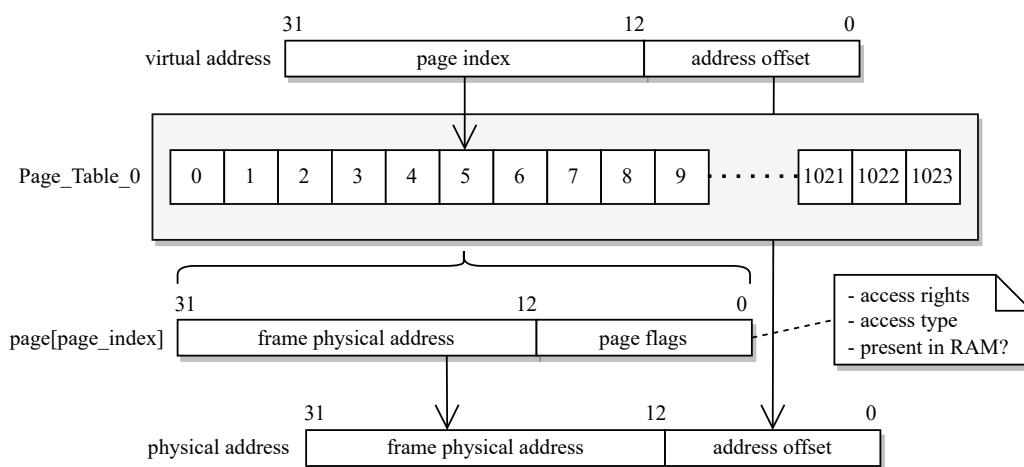
Figure 6.36: Structure of the first-level page table
