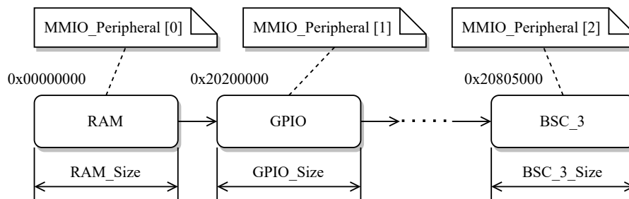
Figure 6.7: Collection of memory-mapped peripherals
