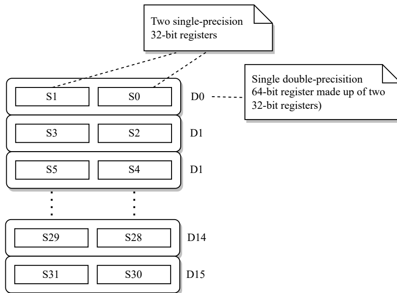
Figure 3.9: Floating-point registers
