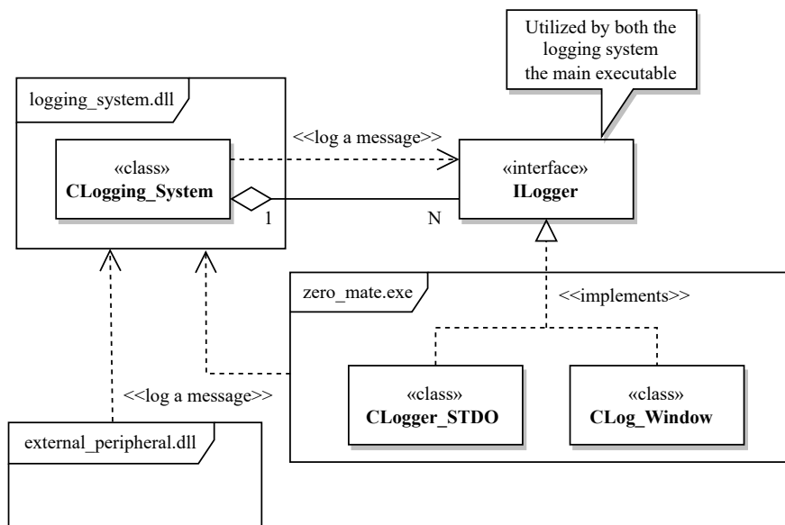
Figure 6.44: Hierarchy of endpoint loggers utilized by the logging system
