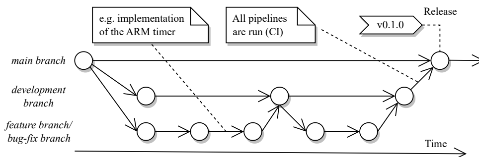
Figure 7.1: Branching strategy of the ZeroMate project 4
