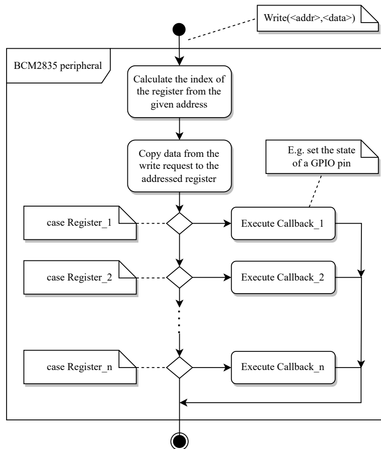
Figure 6.13: Writing to a peripheral's register 8
