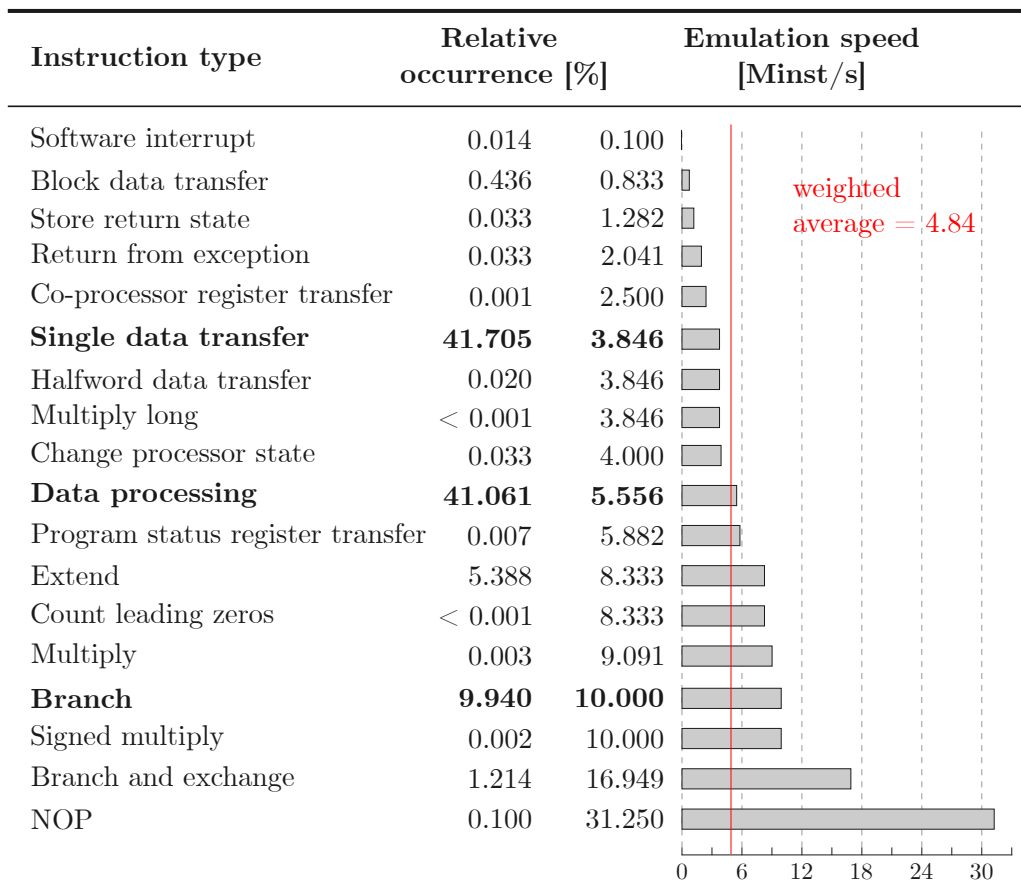
Figure 9.1: ZeroMate's emulation performance of KIV-RTOS
