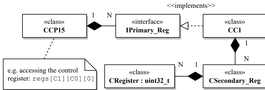
Figure 6.40: Design of the co-processor 15 register hierarchy (uses primary register C1 as an example)
