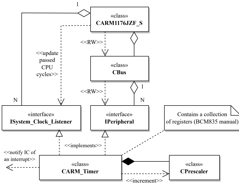
Figure 6.18: Context of the ARM timer component
