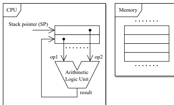
Figure 2.3: Stack architecture
