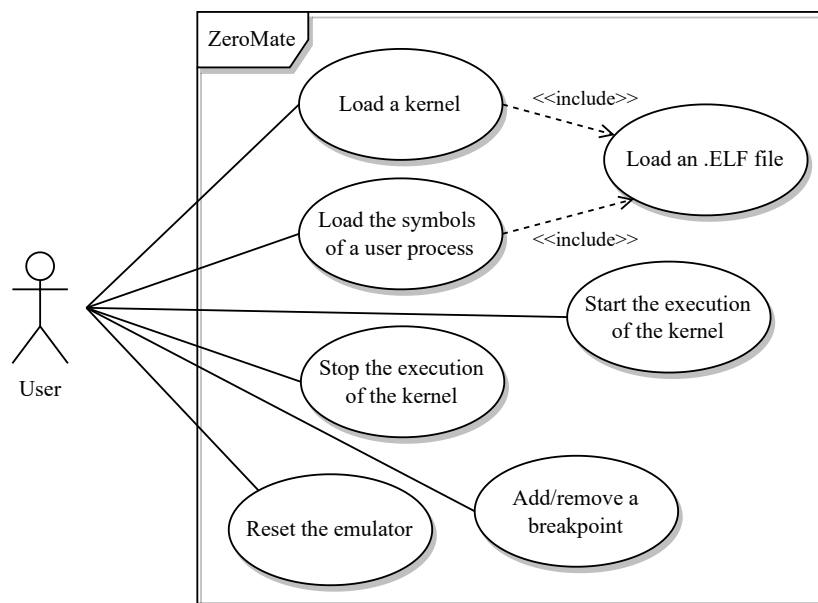
Figure 6.3: Primary use-cases of the ZeroMate emulator
