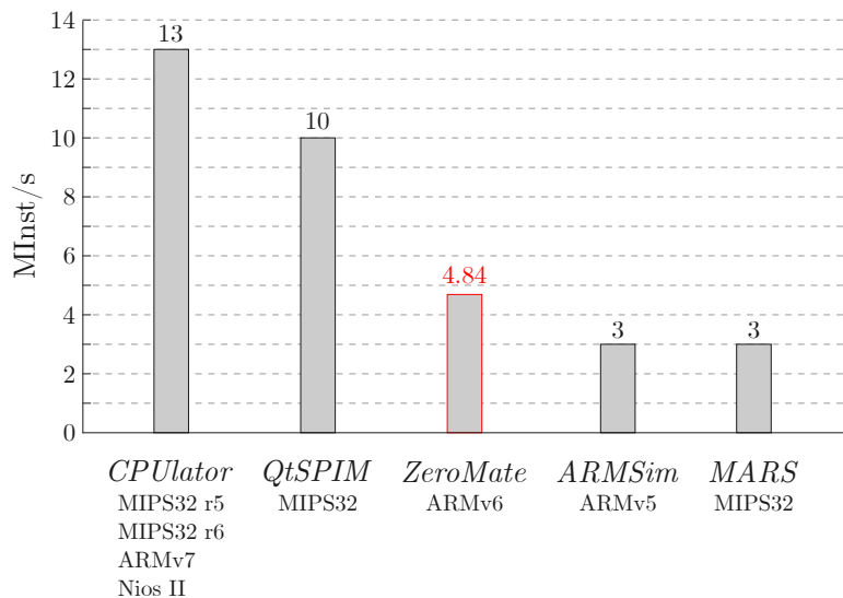
Figure 9.2: Performance comparison of different emulators
