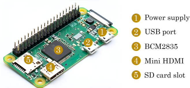
Figure 4.1: Raspberry Pi Zero board
