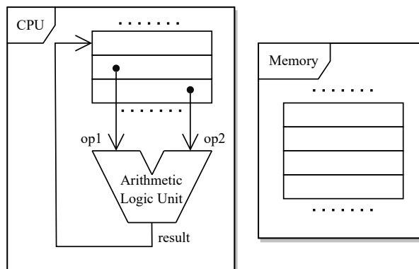
Figure 2.5: Load-store architecture
