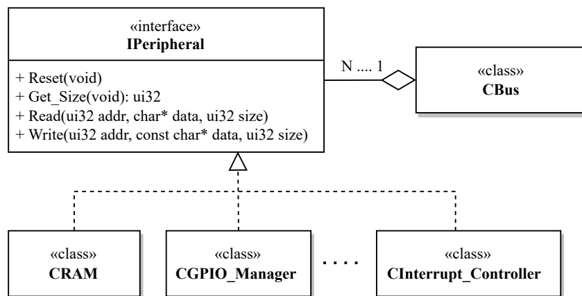
Figure 6.11: Hierarchy of internal peripherals
