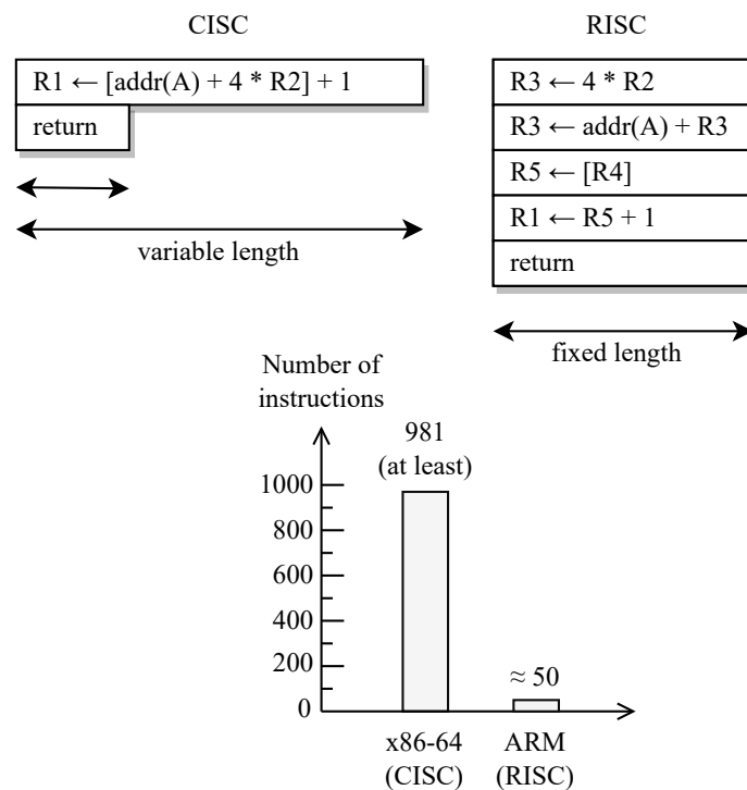
Figure 2.7: Comparison between the RISC and CISC architectures [8]
