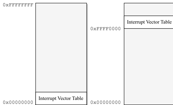
Figure 3.4: Possible locations of the interrupt vector table in RAM
