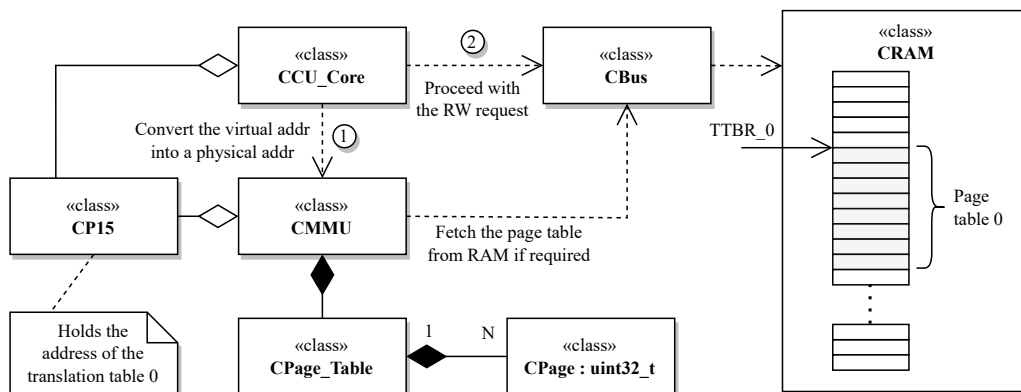
Figure 6.35: Utilization of the MMU when processing a RW request
