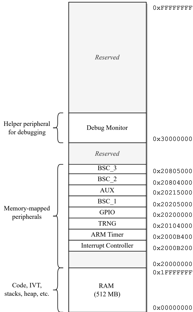
Figure 6.12: BCM2835 physical memory layout emulated by ZeroMate
