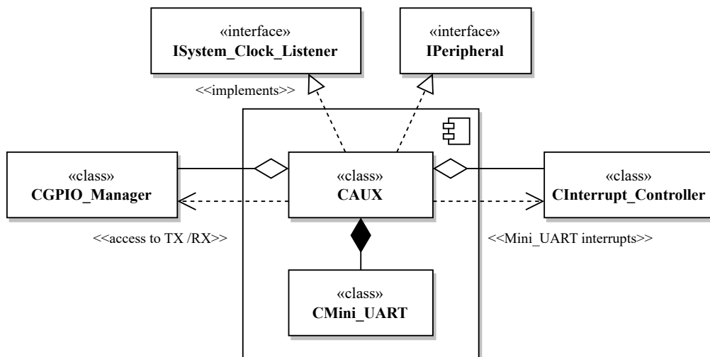
Figure 6.24: Structure of the AUX peripheral
