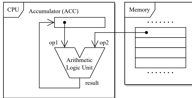
Figure 2.4: Accumulator architecture
