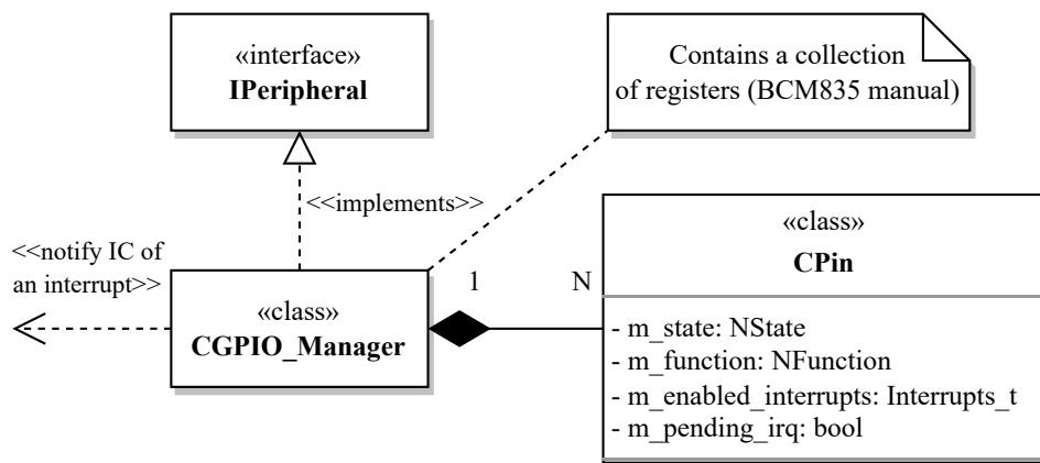
Figure 6.20: Structure of the GPIO manager 14
