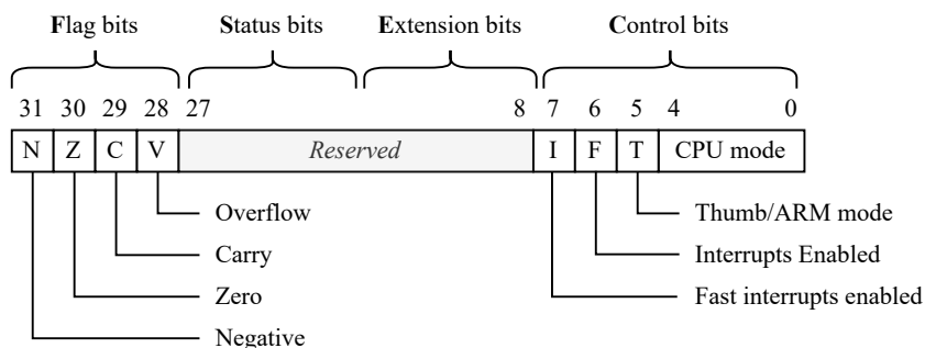
Figure 3.6: Current Program Status Register 4
