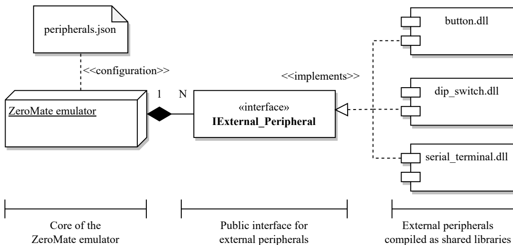
Figure 6.41: External peripheral interface
