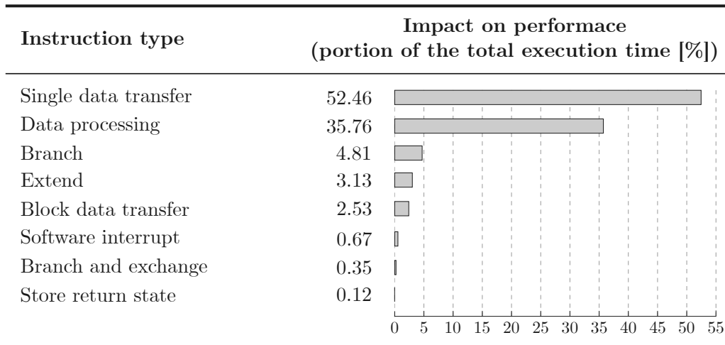
Figure 9.3: Top 8 most performance-affecting instructions 3
