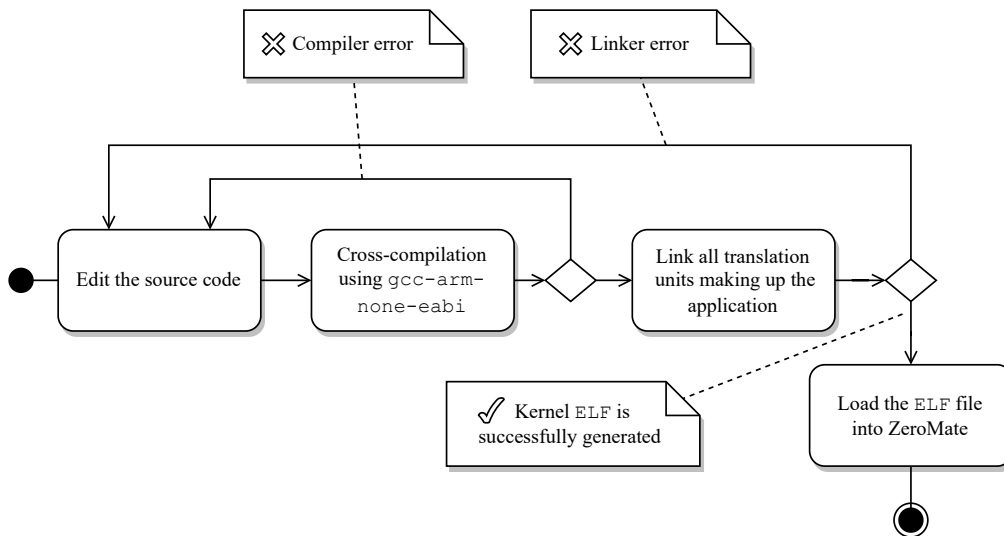
Figure 6.2: Process of building an ELF file (input for the emulator) 2
