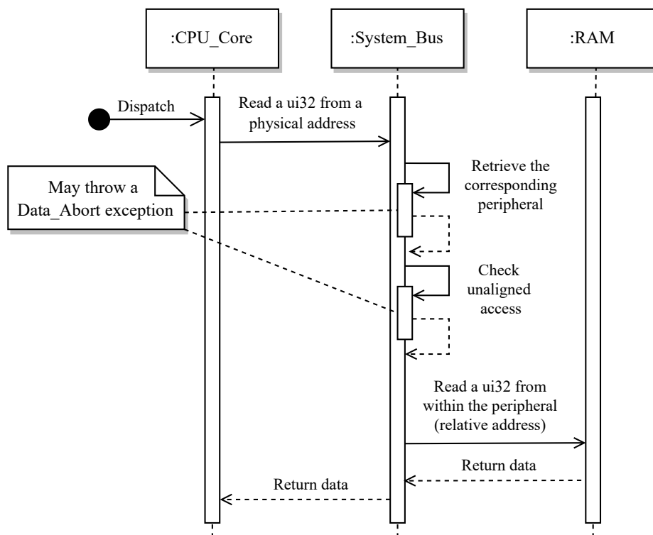
Figure 6.6: Example of a read/write data request issued by the CPU
