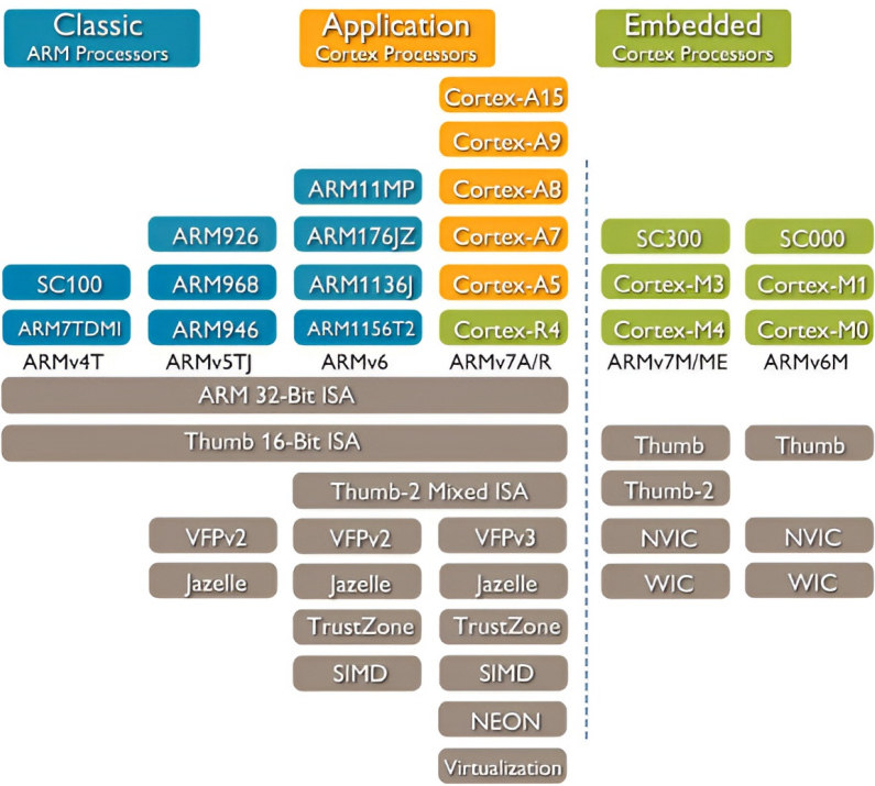
Figure 3.3: Features of different ARM processor cores
