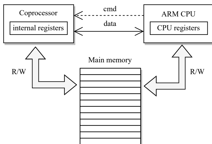
Figure 3.8: Context of an ARM co-processor
